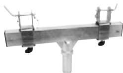
No. 59007080 EUROLITE TAH-35L Truss Adapter for STC-550 Adapter from 150 to 545 mm, 54 mm pin, max. load WLL 1000 kg
