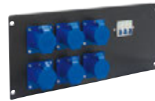
No. 30248900 EUROLITE PDM 5U-6CEE 16A 3pin Power distributor module for rack installation
