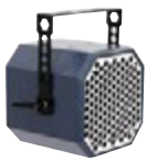
No. 11041174 PSSO PRIME-10CX Coaxial Speaker, 300W Pro PA speaker, 10" woofer, 1" horn, 300 W RMS, 8 ohms
