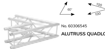
No. 60306540 ALUTRUSS QUADLOCK 6082C-19 2-Way Corner 45°
