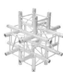
No. 60306590 ALUTRUSS QUADLOCK 6082C-61 6-Way Cross Piece
